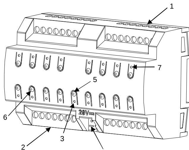
Figura 1. MAXinBOX SHUTTER 8CH
