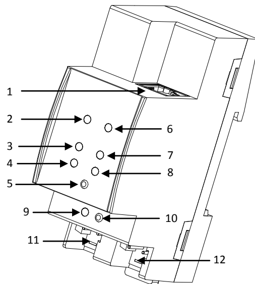
Figura 1. KNX-IP Router
