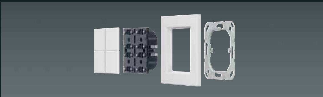
Assembling of the KNX push-button modules with integrated bus coupling unit
